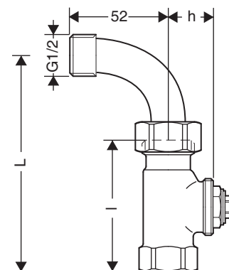
Fig. 11. Straight with swanneck
